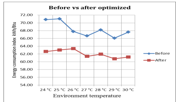
Fig. 9. Comparing energy efficiency.
