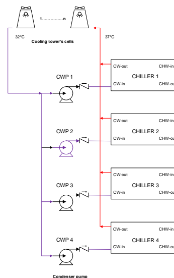
Fig. 1. Condenser water system.
