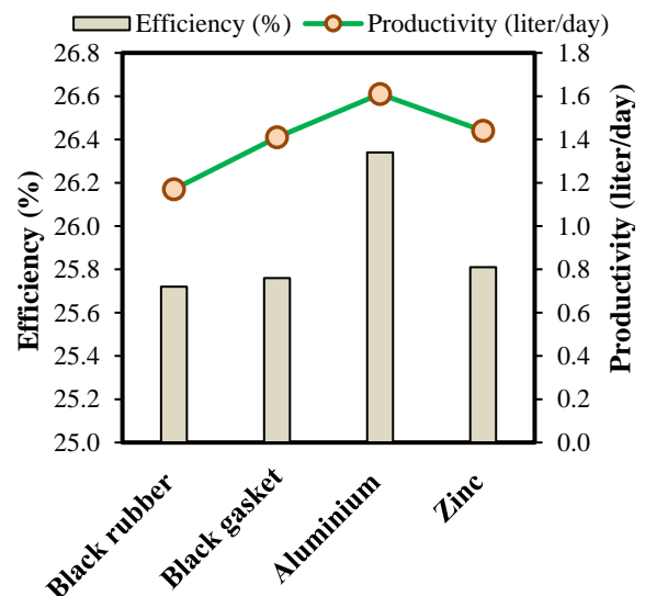
Fig. 9. Comparison between efficiency and productivity of distillation unit with different type of heat absorbers.
