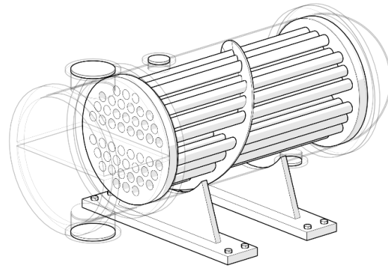
Fig. 6. Configuration of baffles and tubes in isometric view with baffle inclination.
