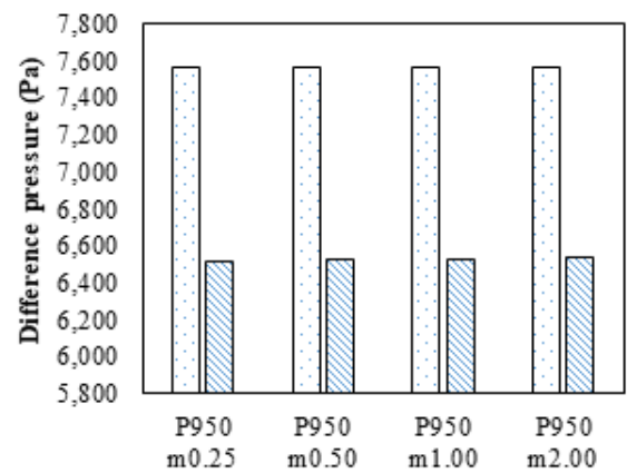
Fig. 24. The difference in pressure of the fluid mass flow rate changes on water.
