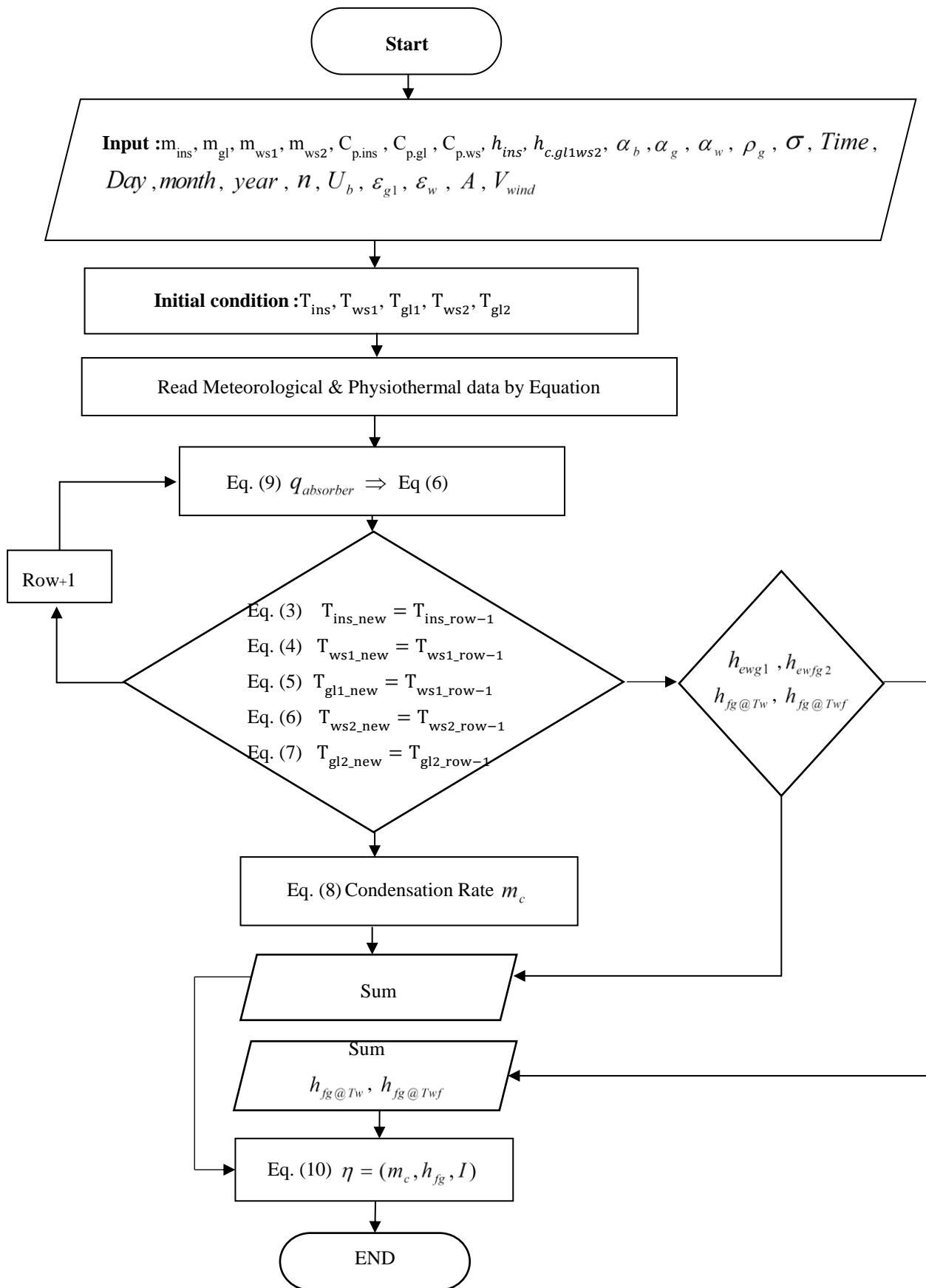
Fig. 1. Using Engineering Equation Solver (EES) to find efficiency of the distillation unit use in the experiment.
