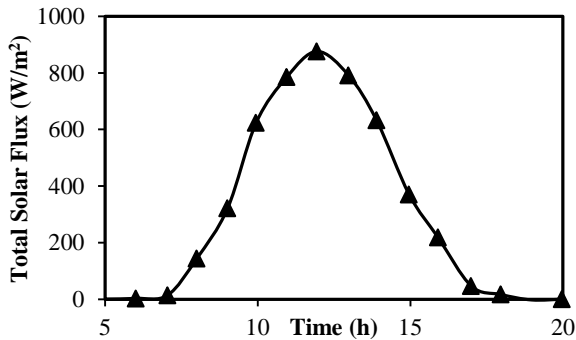
Fig. 3. Monitoring solar flux from 7:00 A.M. to 19:00 P.M for black gasket with 10% heat absorber.
