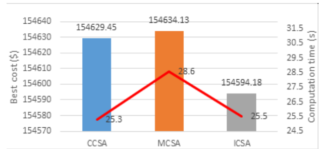
Fig. 3. The best cost and computation time from three methods for system 1.
